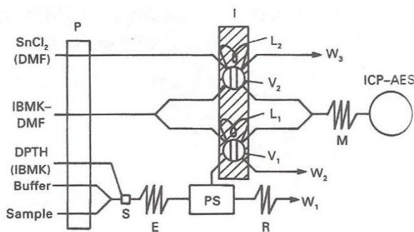
Fig. 1 Schematic diagram of FI manifold for the determination of mercury: P, peristaltic pump; S, segmentor; E, extraction coil; PS, phase separator; R, restrictor (length 50 cm, i.d. 0.5 mm); I, injector; L 1 and L 2 , injection loops; V 1 and V 2 , injection valves; M, mixing coil; W 1 , aqueous phase waste; W 2 , organic phase waste; and W 3 , reductant waste. See text for other details
